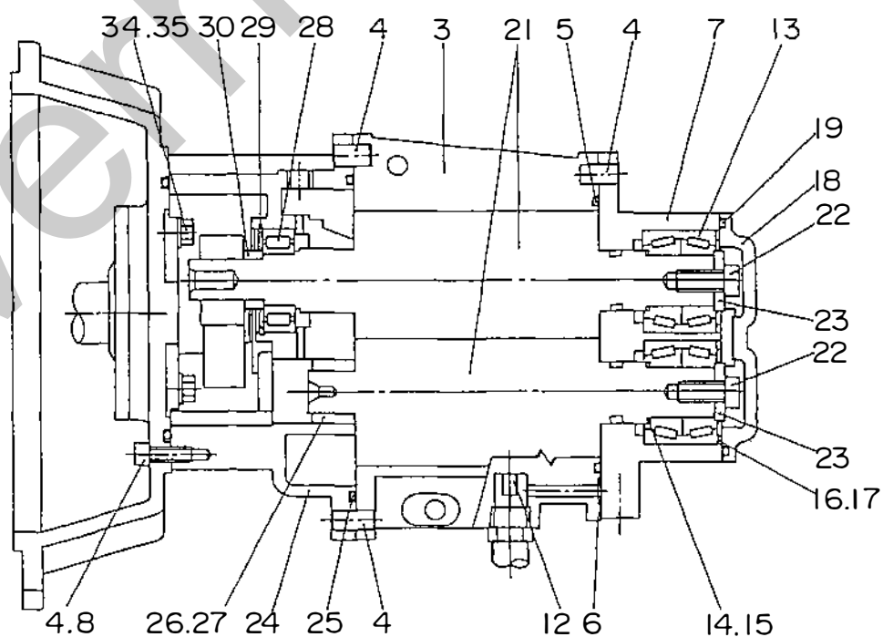
SECTION Y-Y
