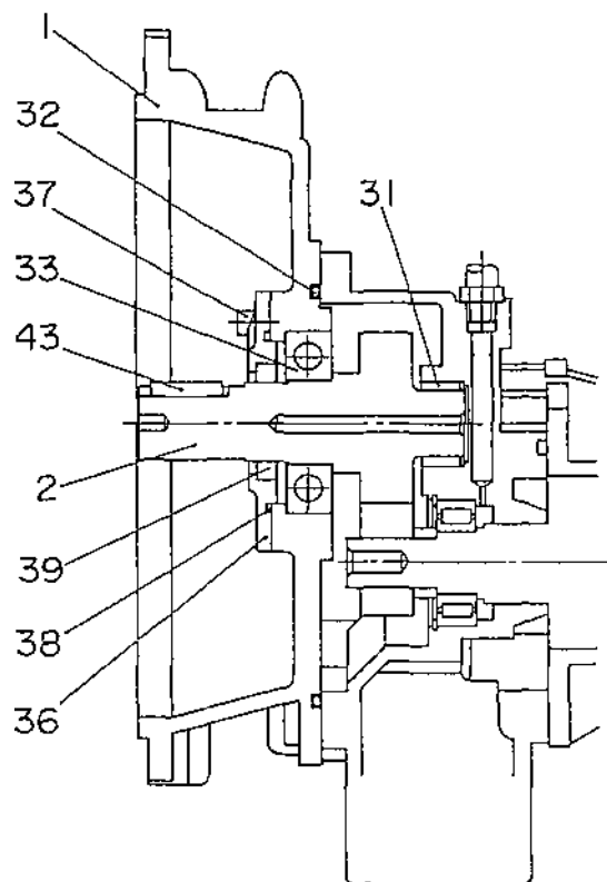
SECTION X-X
